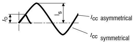
KT4-C2A Max. Let-Through (cut-off) Current, U_e = 400...415V
