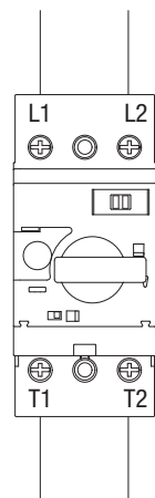
2-Phase KTU7-D-2
