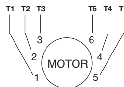
6 LEAD MOTOR CONNECTIONS
