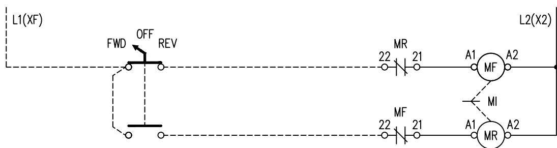
REMOTE FORWARD-OFF-REVERSE SE. SW.
