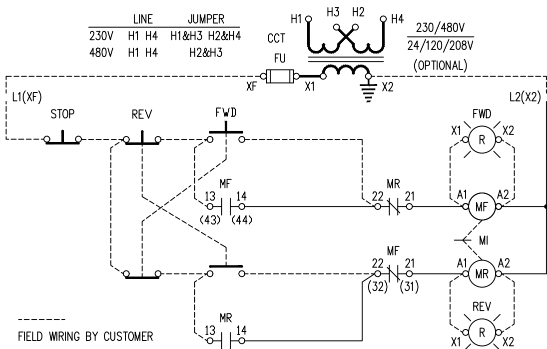
REMOTE FORWARD-STOP-REVERSE PUSHBUTTONS
