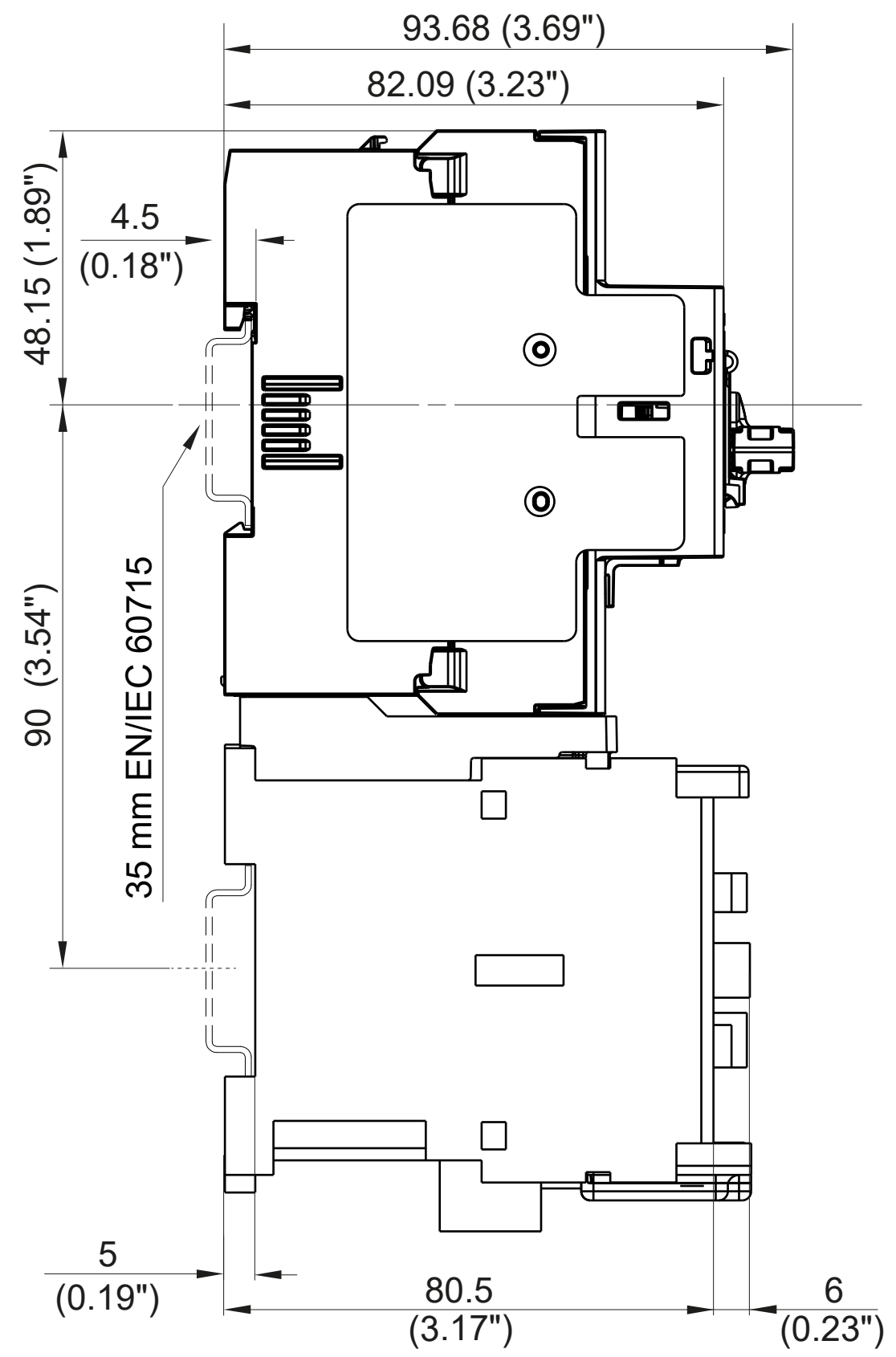
KTA9-40H + KT9-40H-PEC23 + CAU7-9...23
