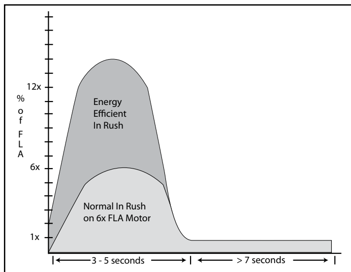
Figure 2: Typical Motor Inrush
