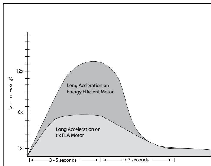
Figure 3: High Efficiency Motor Inrush
