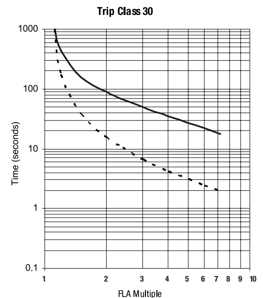
Figure 5: Trip Class 30
