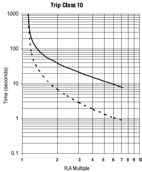
Figure 2: Trip Class 10
