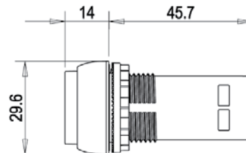
Momentary Pushbutton Device Extended (D7D-E)
