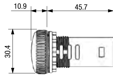
Pilot Light Devices (D7D-P)
