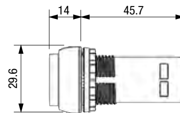
Momentary Pushbutton Device Extended (D7D-E)
