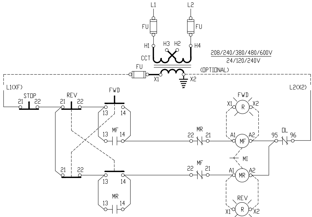
FORWARD STOP REVERSE PB
