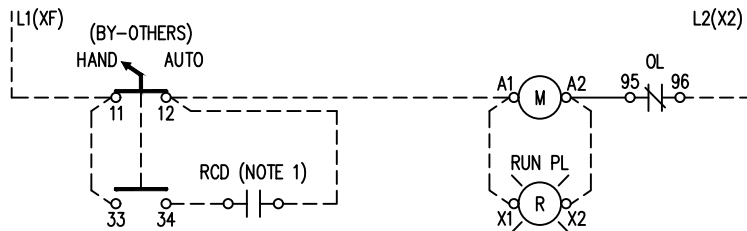
REMOTE HAND-AUTO SELECTOR SWITCH
