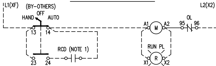
REMOTE HAND-OFF-AUTO SELECTOR SWITCH
