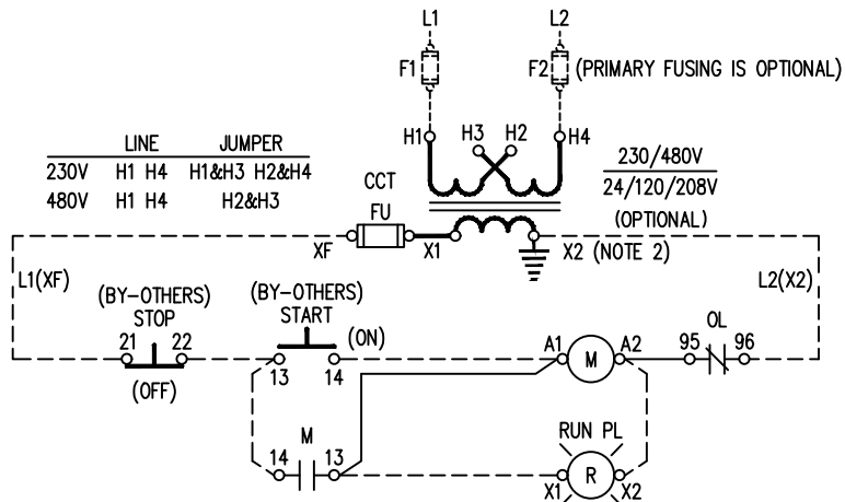
REMOTE START-STOP PUSHBUTTONS
