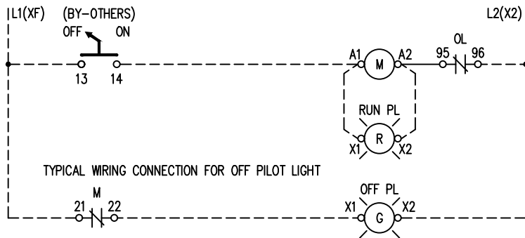
REMOTE OFF-ON SELECTOR SWITCH
